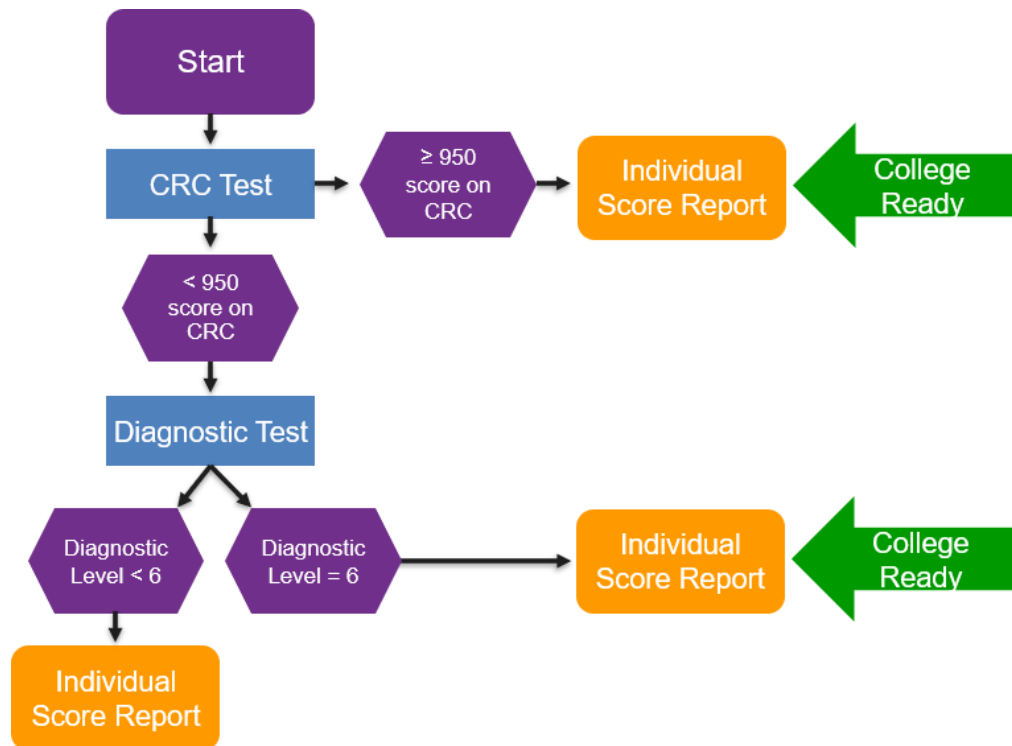
Figure 1. Routing flow
